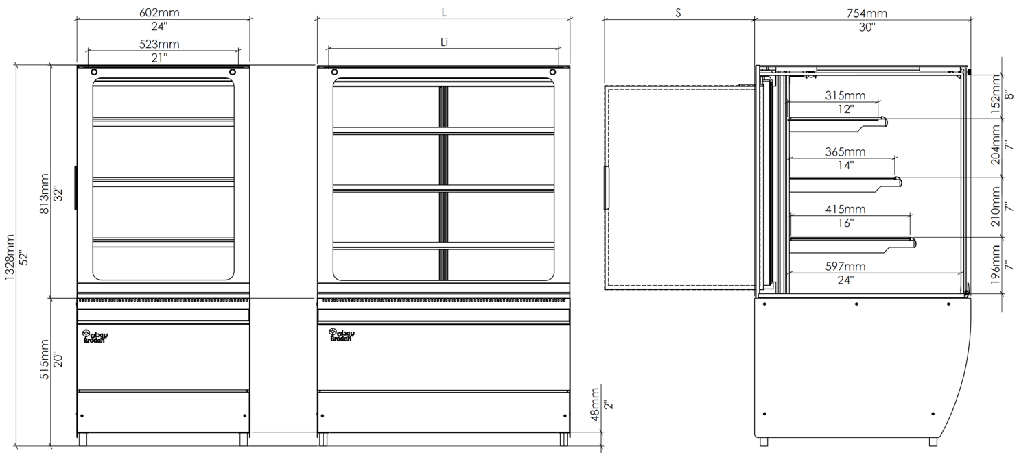
600 Front Elevation
