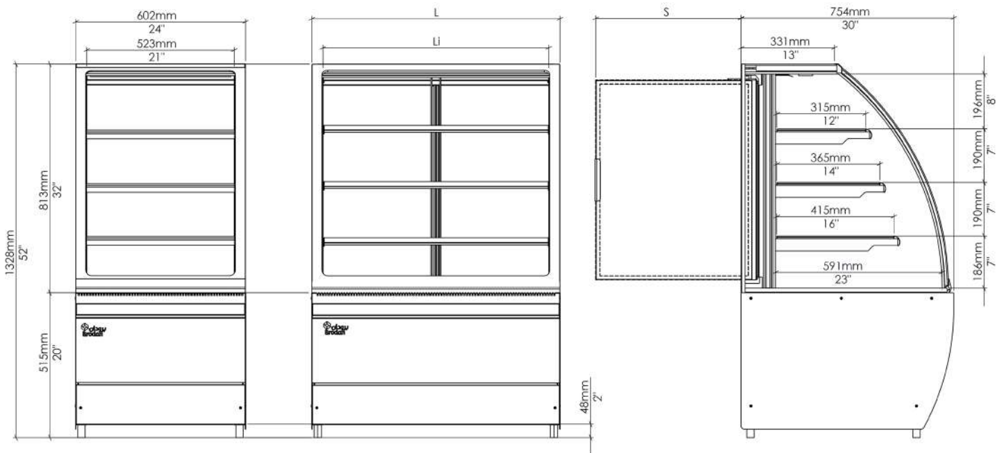
600 Front Elevation
