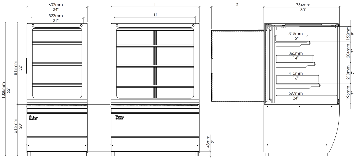
600 Front Elevation
